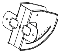
A6 : Back Mount Elevation (1ea)
